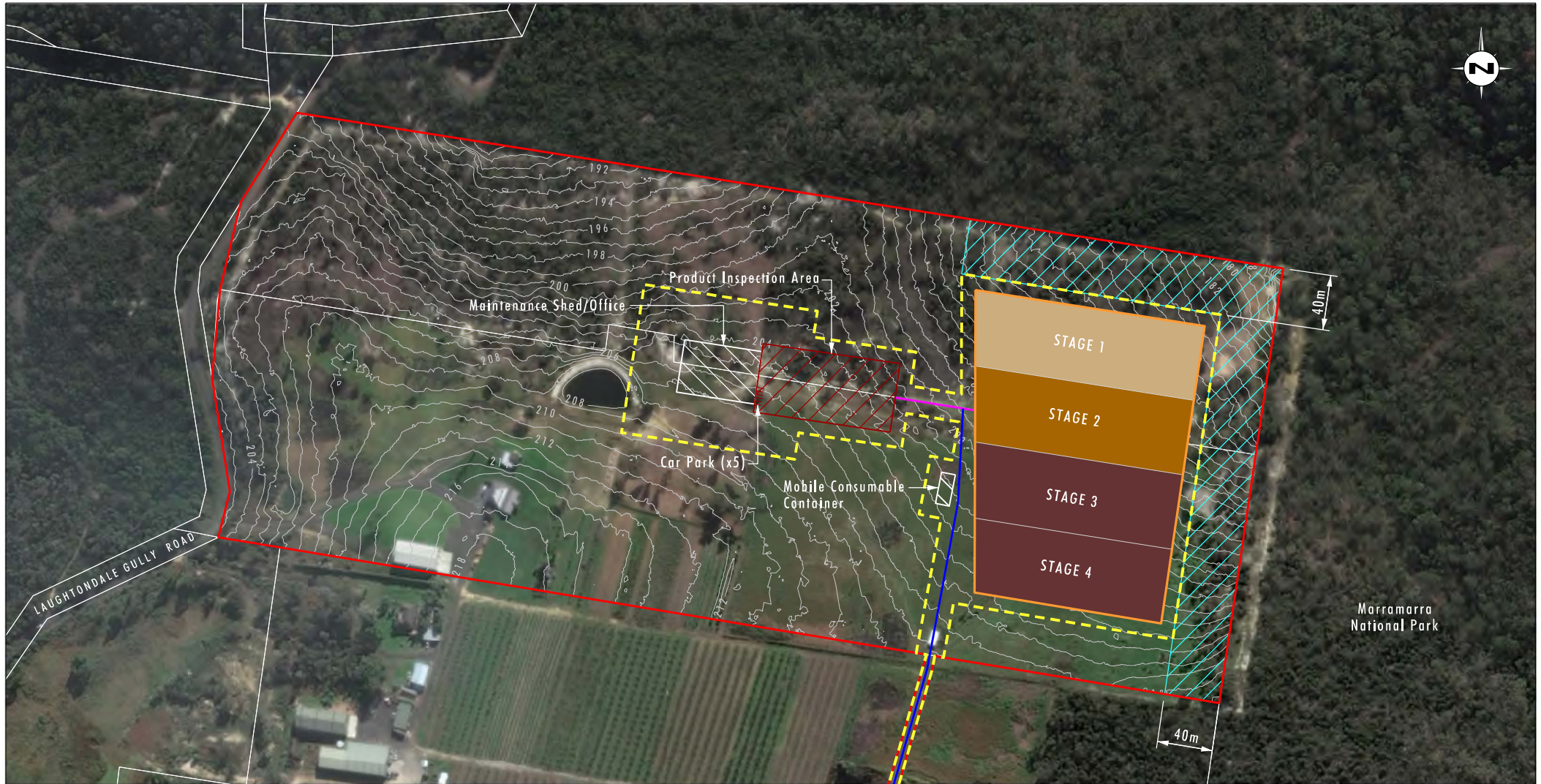
FIGURE 3.6 Indicative Quarry Plan - Year 7
